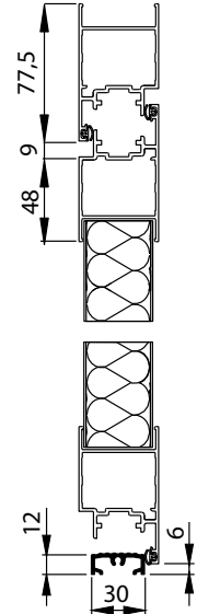
DoorPro 45, Profile Dimensions
